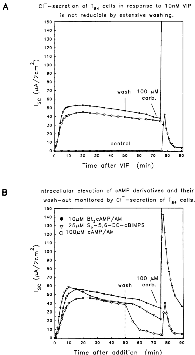
Fig. 2. Activation of \text{Cl}^- secretion by \text{T}_{84} cells mounted in Ussing chambers (see text for details). A , Extracellular basolateral application of VIP at time 0 and comparison of experiments with a wash procedure (●), as indicated, or without wash (○) (three experiments each). ▽, Control response to carbachol ( carb. ) alone (control experiments). B , Extracellular basolateral application of various membrane-permeant derivatives of cAMP in submaximal doses. Fifty minutes after activation the cells were washed and the decrease of \text{Cl}^- secretion was monitored. Twenty-five minutes after the wash (i.e., 80 min after the activation) 100 \mu\text{M} carbachol was added to induce synergistic \text{Cl}^- secretion in all experiments. In the case of \text{bt}_2\text{cAMP/AM} , the I_{\text{sc}} exceeded 200 \mu\text{A}/2\text{cm}^2 and the voltage clamp had to be shut off. All traces represent the mean of at least three experiments in duplicate.
