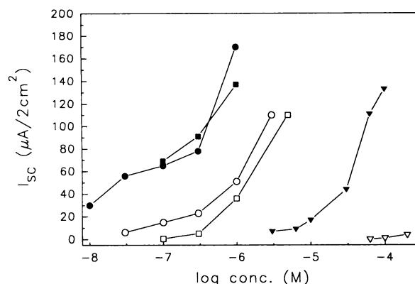
Fig. 4. Dose-response relationship for the net synergistic \text{Cl}^- secretion induced by carbachol without wash (closed symbols) or 25 min after the wash (open symbols) (three to seven experiments each) for monolayers incubated with cAMP/AM (inverted triangles), \text{S}_p -DCI-cBIMPS (squares), or \text{bt}_2\text{cAMP/AM} (circles). The net synergistic \text{Cl}^- secretion is defined as the peak response minus the level of \text{Cl}^- secretion at the moment of carbachol addition minus the standard response to carbachol alone ( 43 \pm 5 \mu\text{A}/2\text{cm}^2 ) (three experiments).
