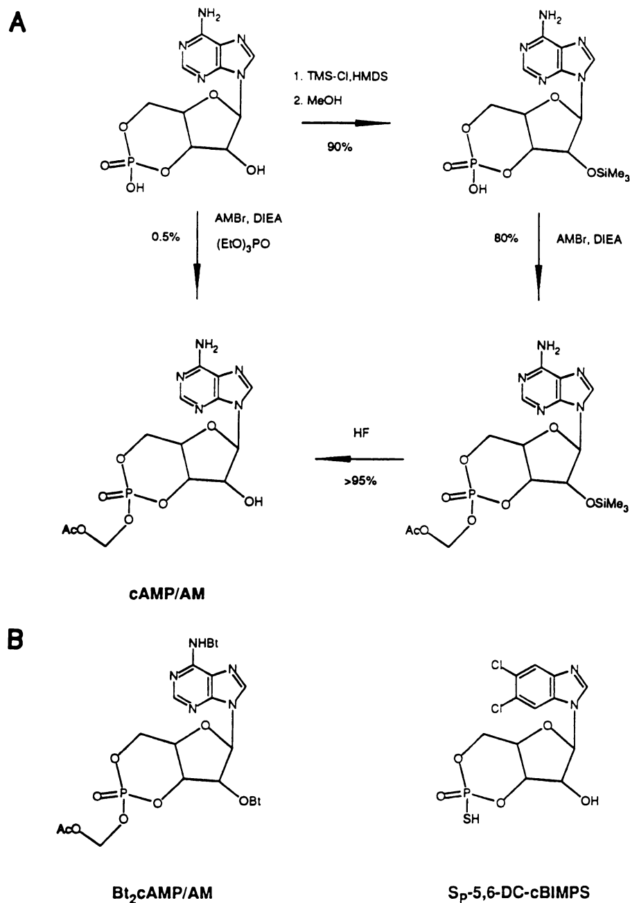
Fig. 1. Synthesis pathway to cAMP/AM (A) and the structures of bt 2 cAMP/AM and S p -5,6-DCI-cBIMPS (B). HMDS , hexamethyldisilazane; MeOH , methanol; Me , methyl; Et , ethyl.
