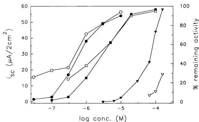
Fig. 3. Dose dependence of \text{Cl}^- secretion. Experiments were performed as depicted in Fig. 2. Data points for the dose dependencies of \text{Cl}^- secretion were taken 12 min after activation (closed symbols) and those for the reduction of \text{Cl}^- secretion after the wash were taken 12 min after the wash (open symbols) for cAMP/AM (inverted triangles), \text{S}_p -5,6-DCI-cBIMPS (squares), or \text{bt}_2\text{cAMP/AM} (circles). All experiments were performed at least three times in duplicate.
